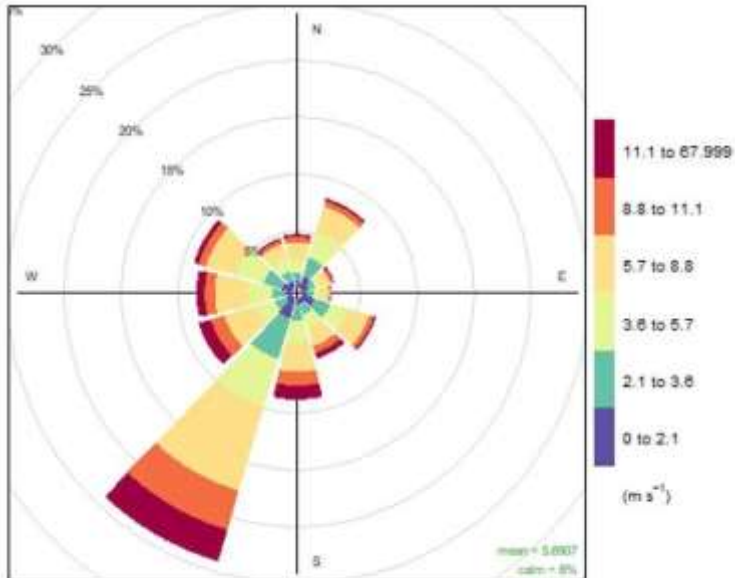
Figure 2.3 2016-2020 Windrose from Cambridge/Mildenhall
