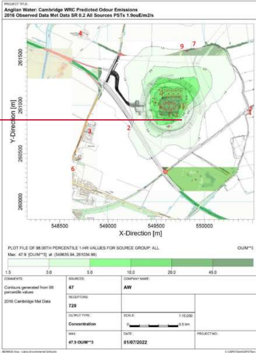
Figure 4-5: Odour modelling result for Scenario 1
