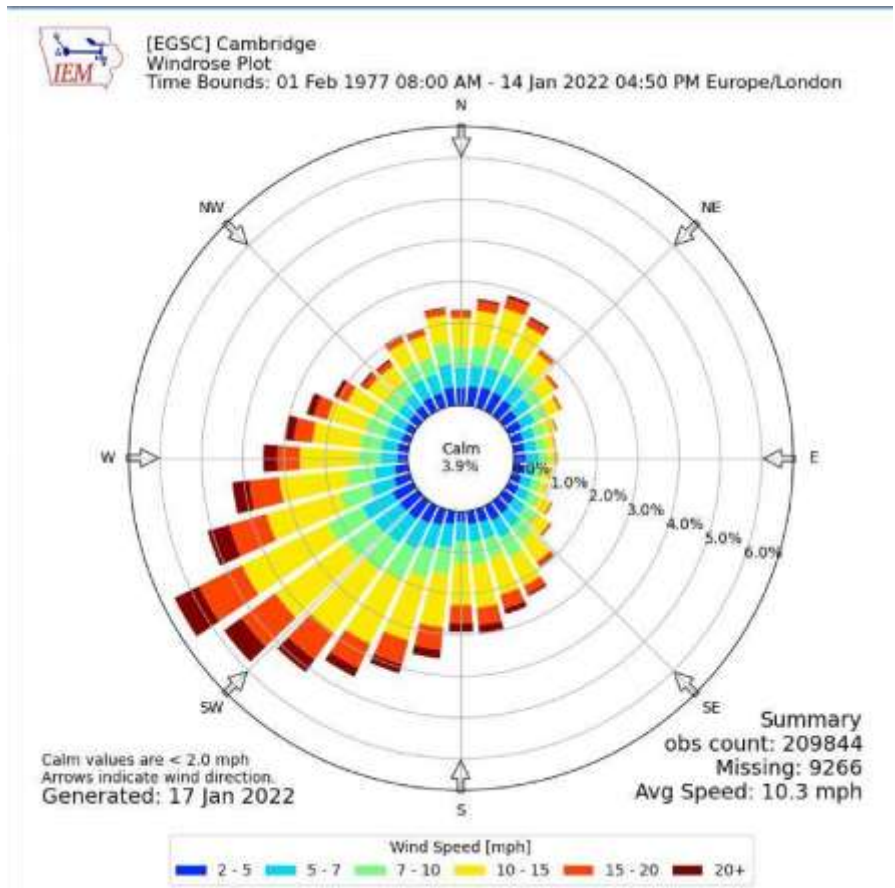
Figure 7: Cambridge Windrose Plot – Cambridge Airport
