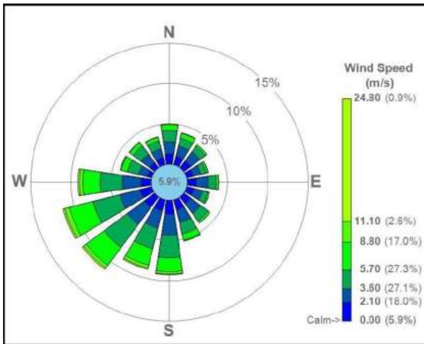
Figure 3-1: Cambridge/Mildenhall MET data windrose average 2016 to 2020.
