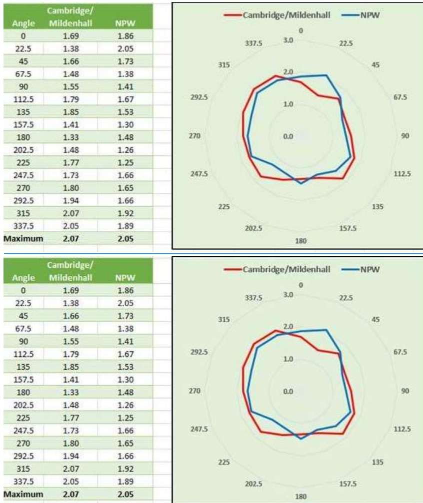
Figure 4-1: NWP and observed MET data comparison of the maximum 98 th percentile (2016 to 2020).
